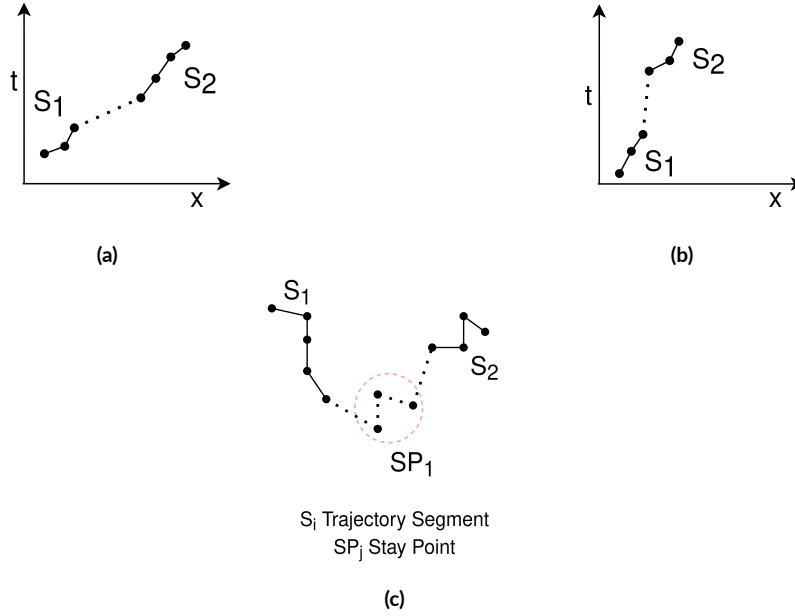
Figure 2.2: (a) Segmented trajectories by spatial gaps [1] (b) Segmented trajectories by temporal gaps [1] (c) Segmented trajectories by stay points [2]
