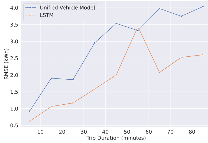
Figure 4.7: Prediction RMSE (kWh) by duration of the trips
