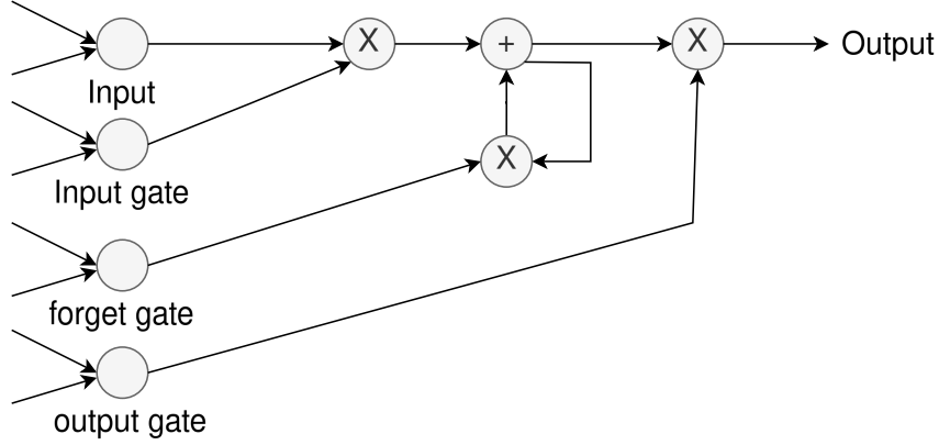
Figure 2.5: Illustration of an LSTM architecture [4]
